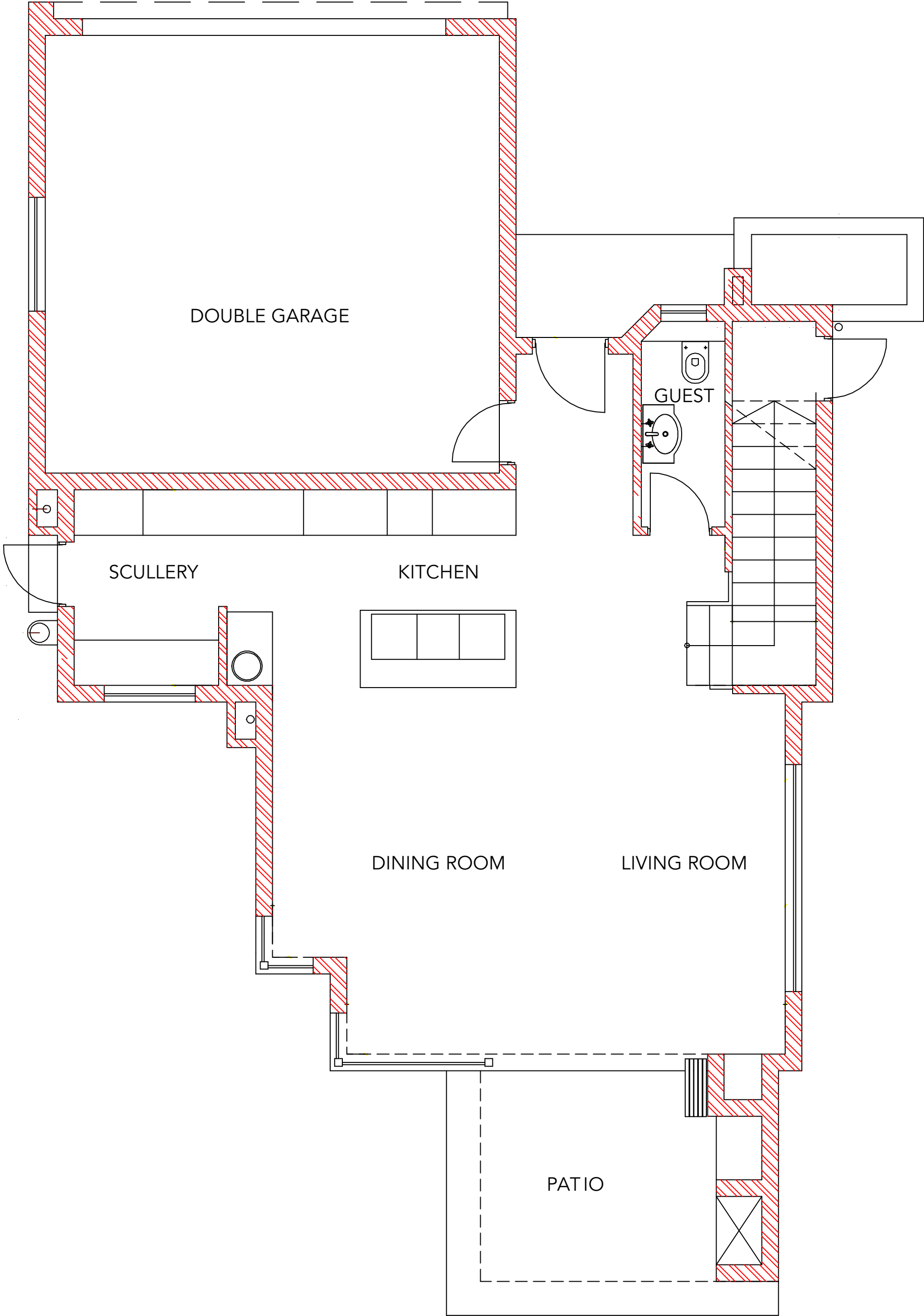
GROUND FLOOR PLAN - 125m²
