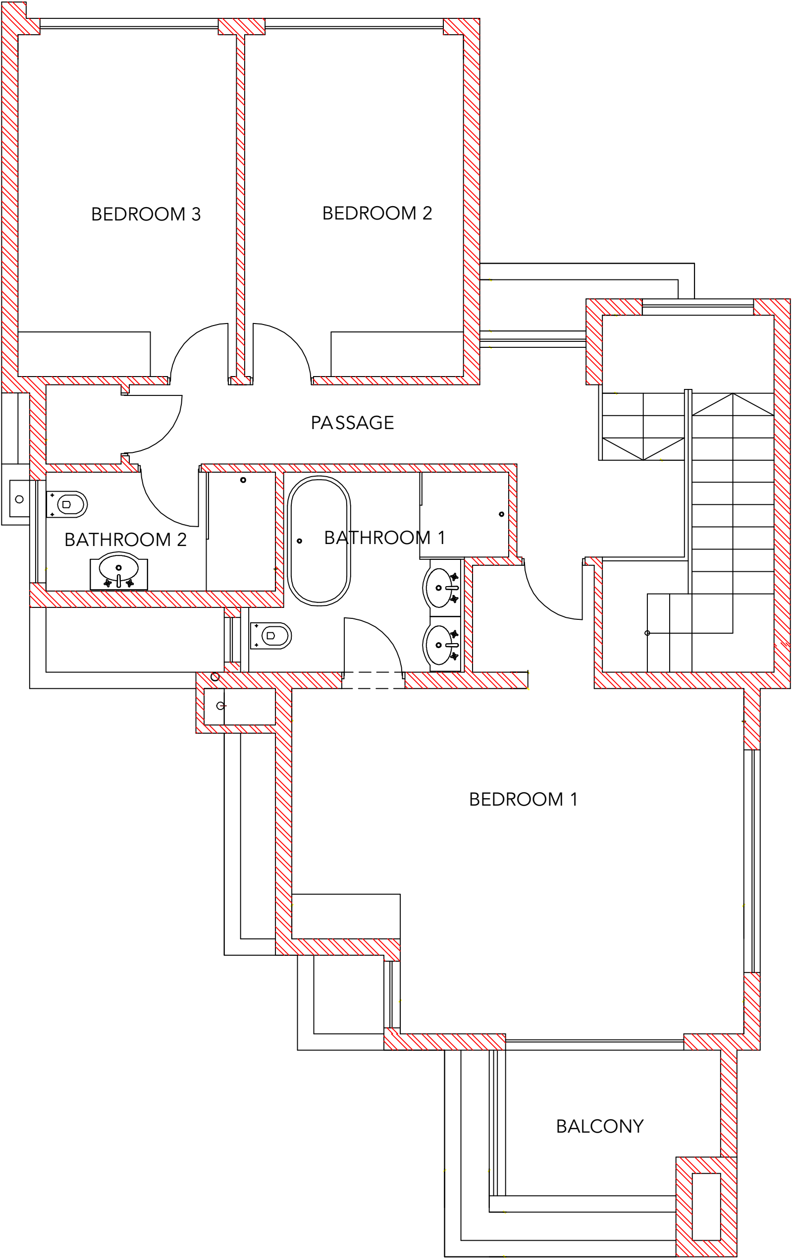
FIRST FLOOR PLAN - 94m²
