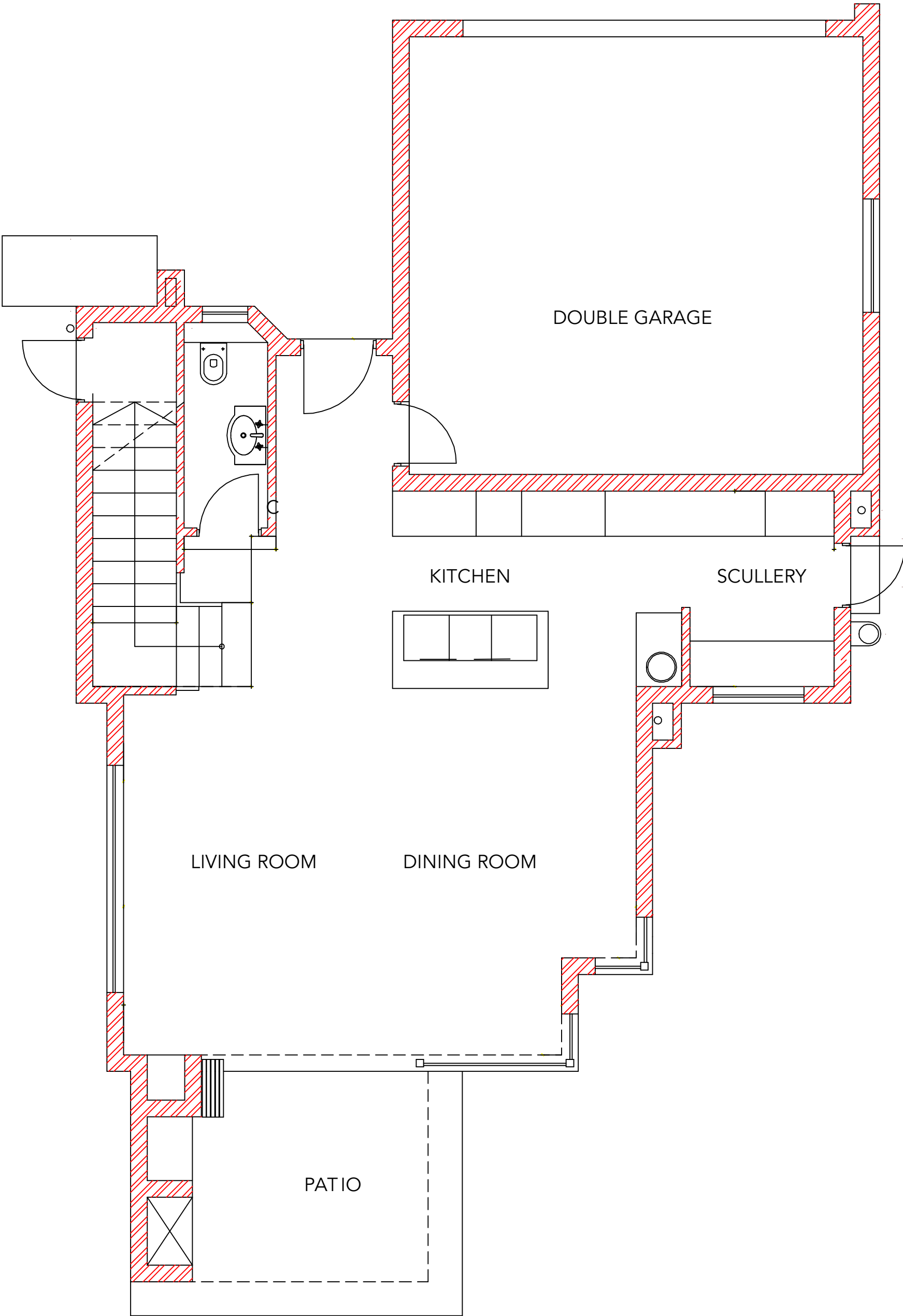
GROUND FLOOR PLAN - 125m²
