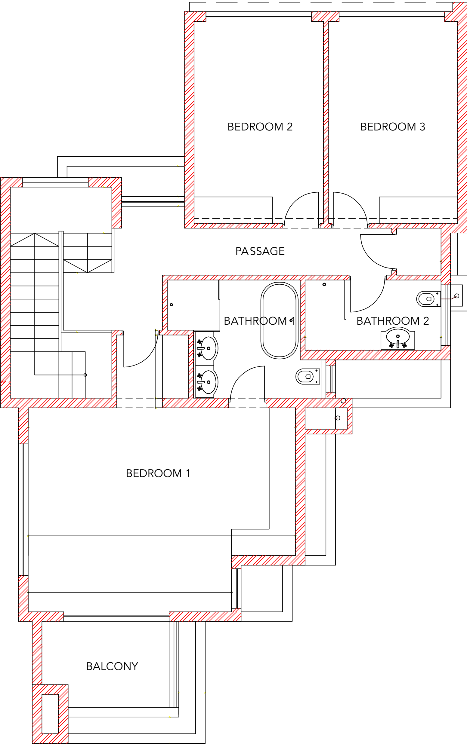
FIRST FLOOR PLAN - 94m²
